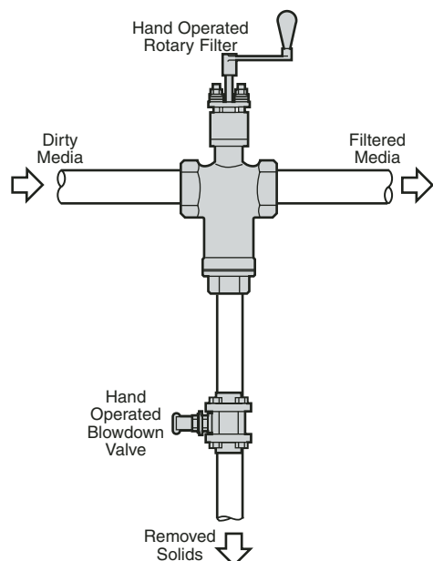
Figure II-97 Hand Operated Rotary Filter
