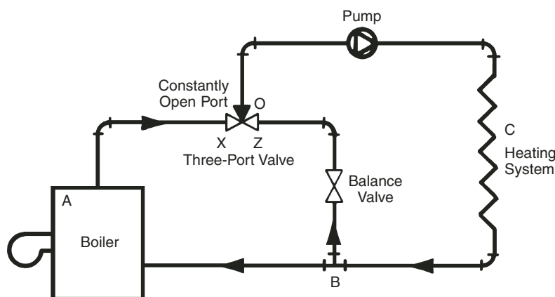
Figure 43 Three-Port Mixing Valve in a Closed Circuit (Constant Volume, Variable Temperature)
